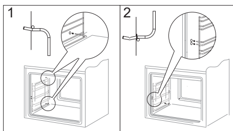
Inserting side racks
