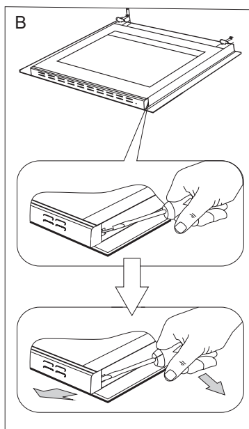
Lifting the hinge security tags
